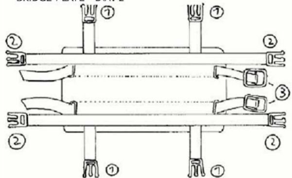
BRIDGE PLATE - DIA. 2
